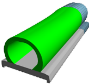
Co-extrusion of soft (green) and dense (grey) rubber for automotive application
