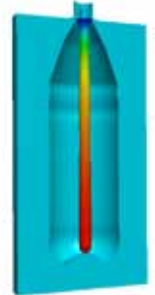
Polyflow makes it possible to study the behavior of plastics and other materials, such as this example of injection stretch blow modeling using shell elements. The image shows thickness distribution.
