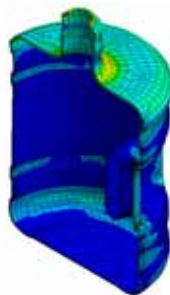
Simulation helps companies to reduce product failure risk early in the design cycle by providing insight into critical parameters/characteristics, such as material distribution (left) and top load stress distribution (middle) in a five-gallon blow-molded water cooler bottle (right).
